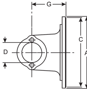
BEARING PLATE
