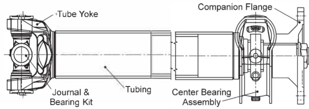
Flange connection design
